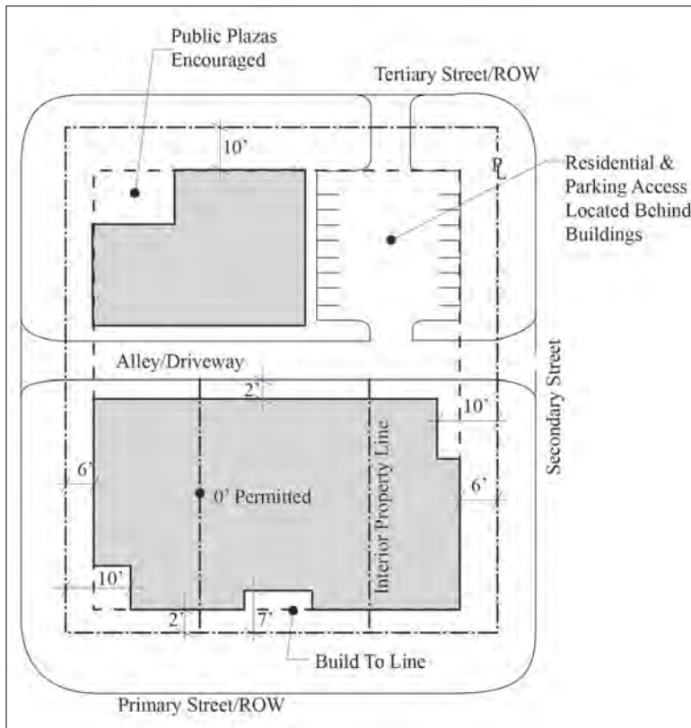
Figure 20.225-2 MU-1 Development Standard Diagram
