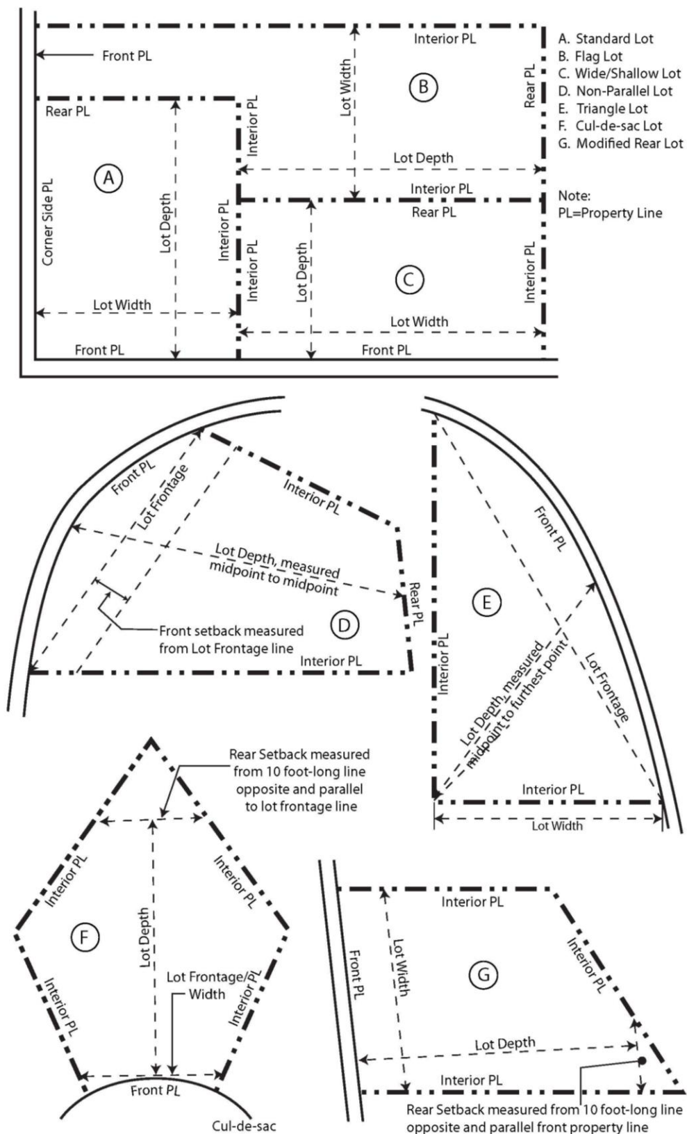
Measuring Lot Size and Setbacks, Standard and Irregular Lots
