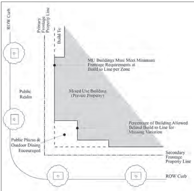
Figure 20.225-3 Build-To Line Diagram
