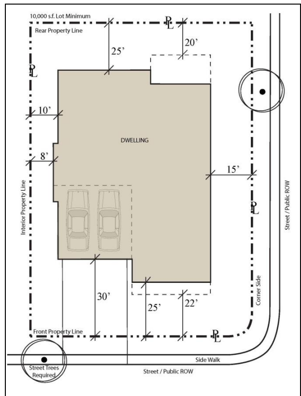
Figure 20.215-2 R-1-10 Zone Development Standards See Table 20.215-3 for standards.
