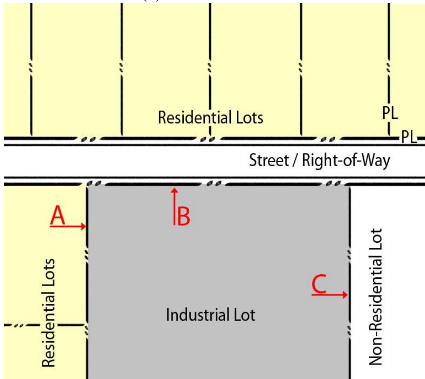
Figure 20.230-4 Additional Setbacks from Residential
