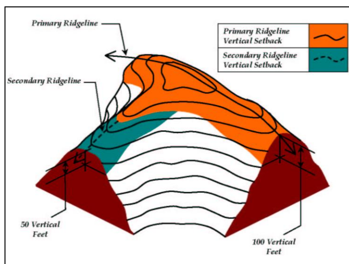
Figure 20.260-4 Illustration of Vertical Ridgeline Setbacks
