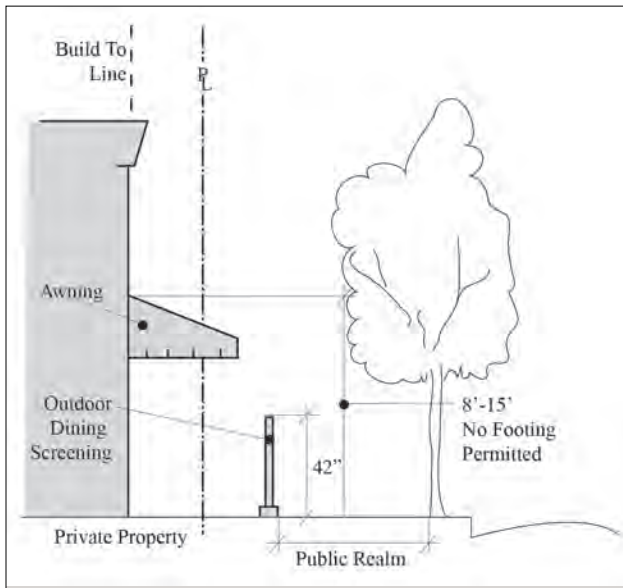
Figure 20.225-8 Setbacks and Encroachments
